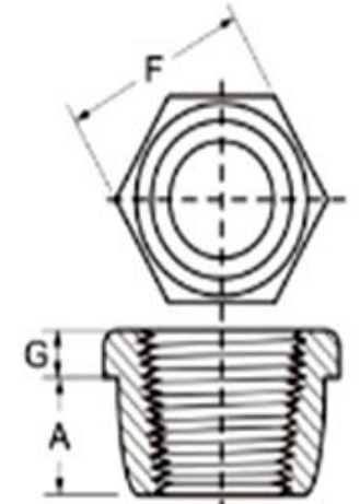
Hex Head Bushing
