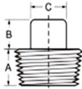
Square Head Plug
